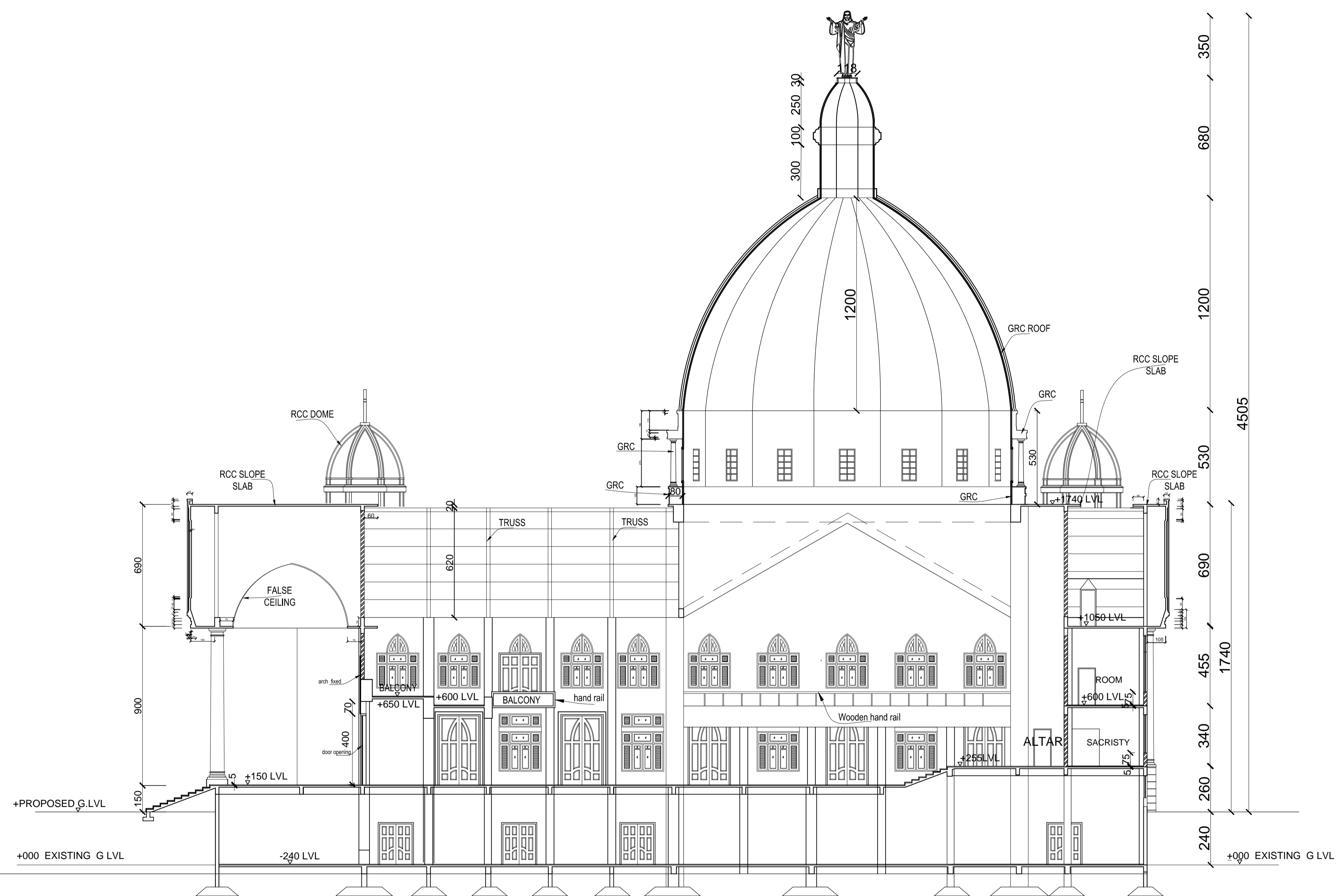
SECTION G G SCALE 1:100
