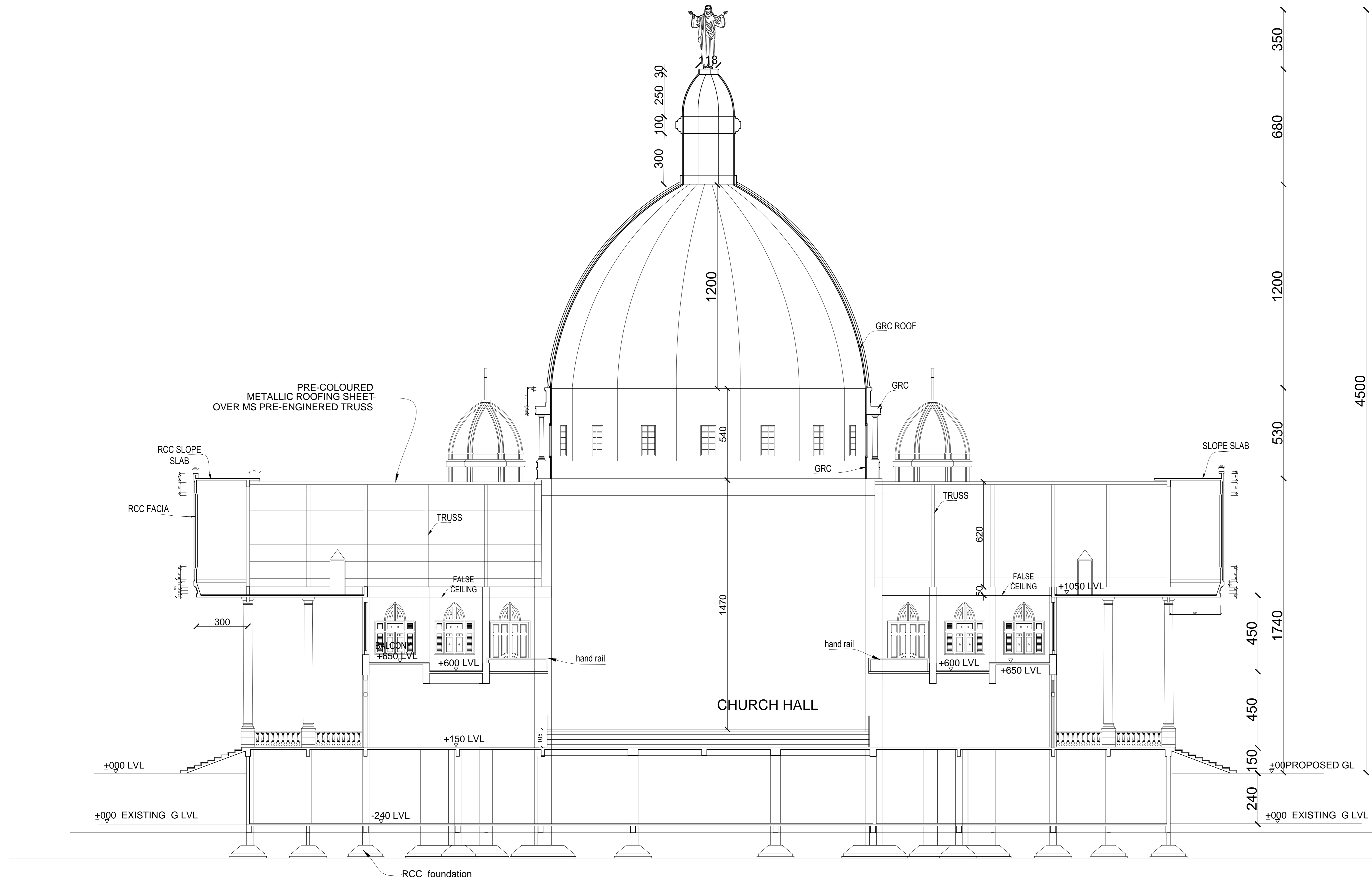
SECTION E E SCALE 1:100
