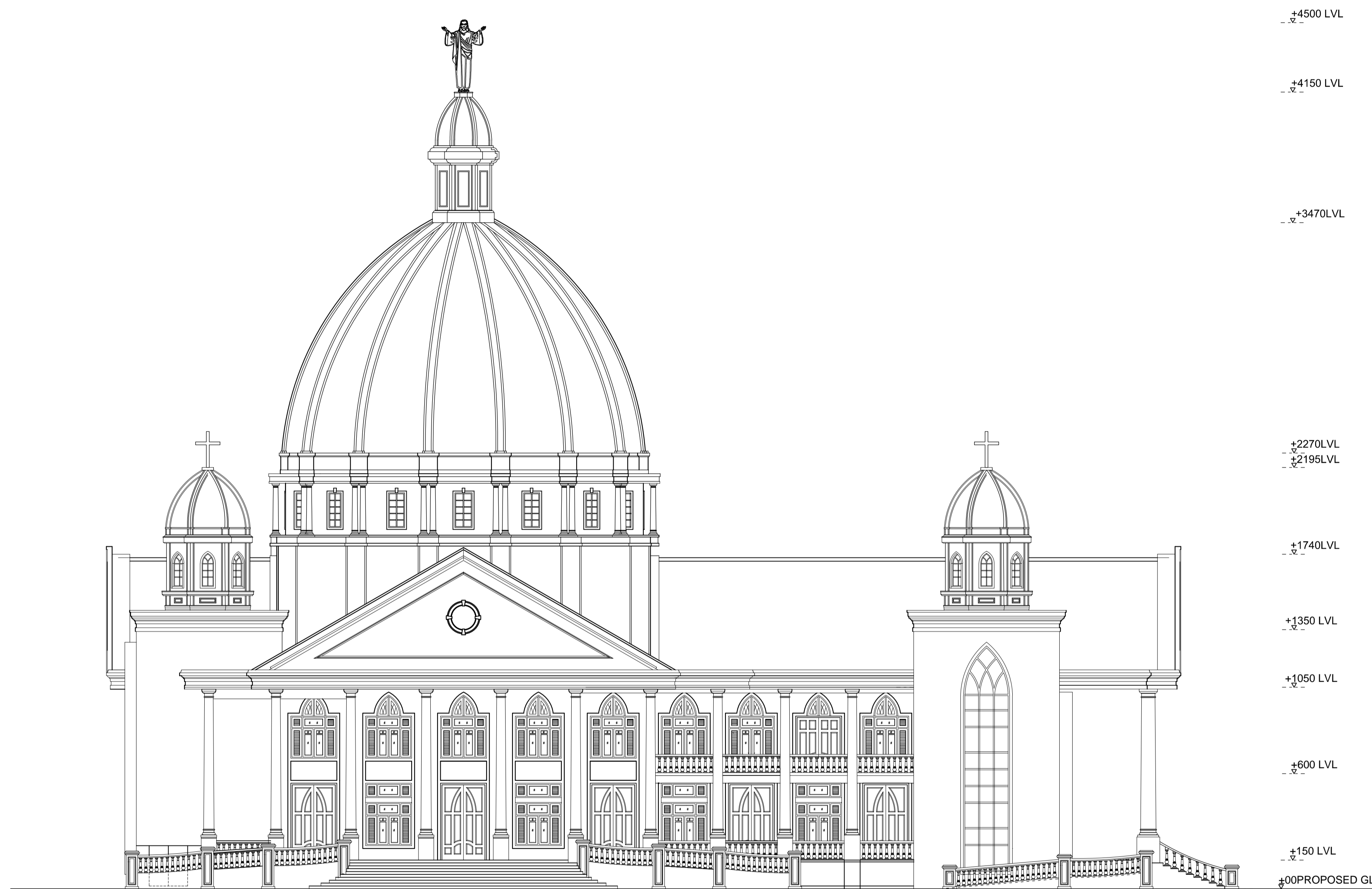
NORTH SIDE ELEVATION SCALE 1:100
